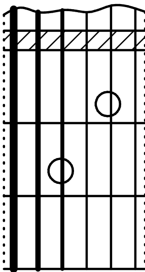
x Am7
