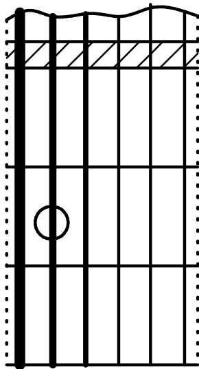
Em7
